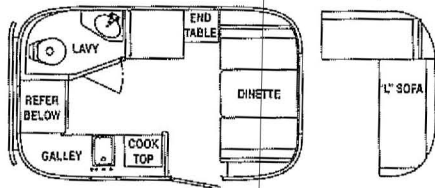
Model 16C Bambi
