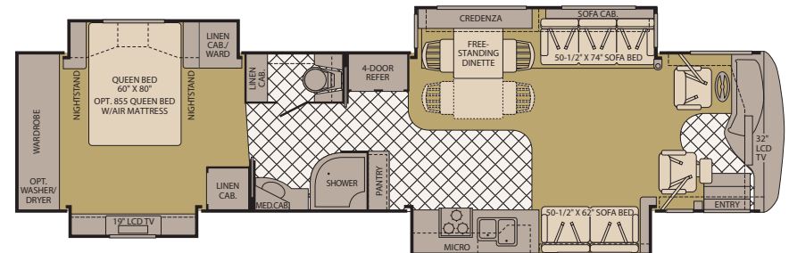
42N Quad Slide-Out
