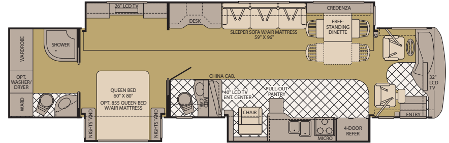
42K Full-Wall Slide Triple Slide-Out
