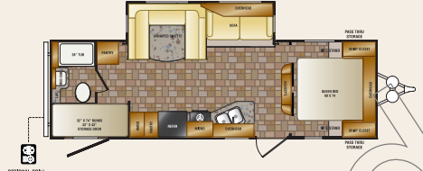
ZT26BL TRAVEL TRAILER
