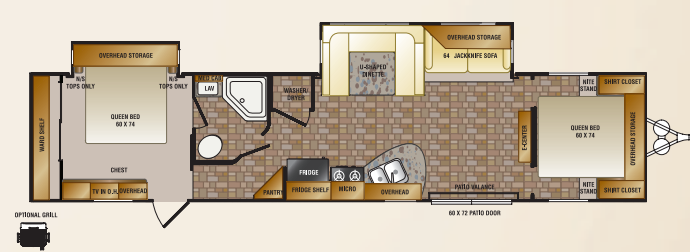
ZT39BH TRAVEL TRAILER
