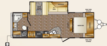
ZT25RB TRAVEL TRAILER
