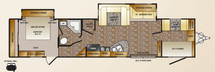
ZT39BH TRAVEL TRAILER
