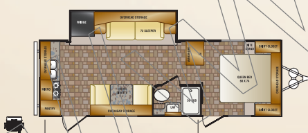
ZT25SB TRAVEL TRAILER
