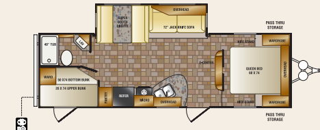
ZT26BH TRAVEL TRAILER
