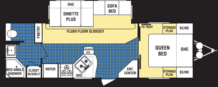
FS260F-DSL
