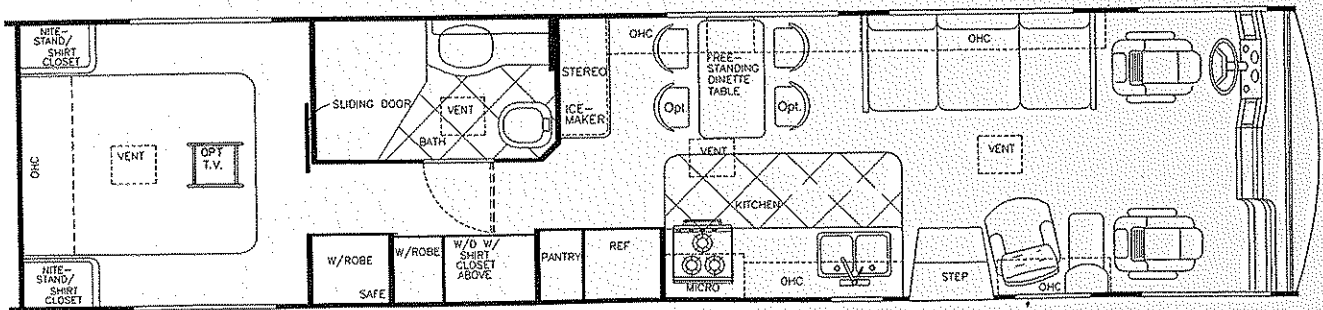
Model 8380 DIESEL
