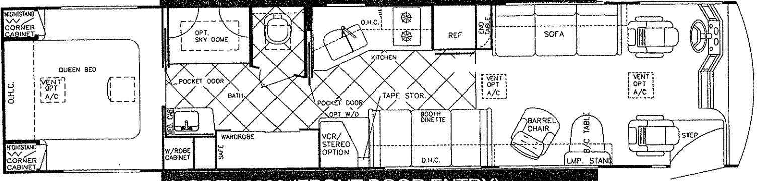
MODEL 8390 (FRONT DOOR ENTRY)
