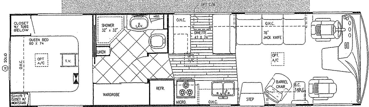
Model 8352 MGB (Approx. 34'6" x 101' Wide)
