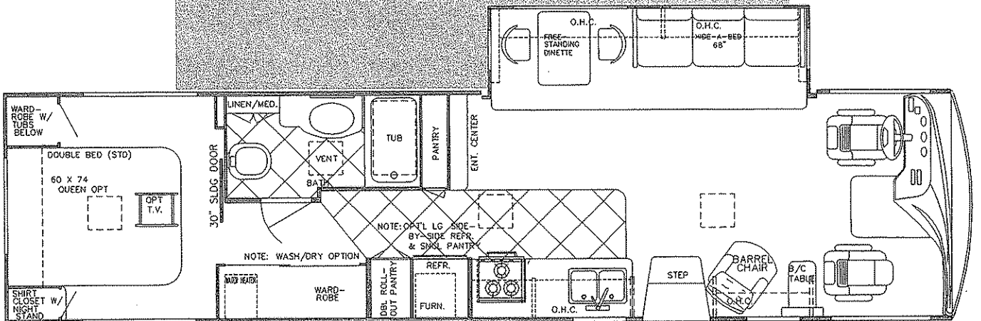
Model 8362 MXG (Approx. 37'6" x 101' Wide)
