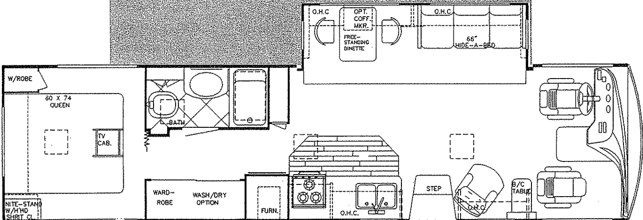
Model 8342 SYG (Approx 34'-8" 95" Wide)
