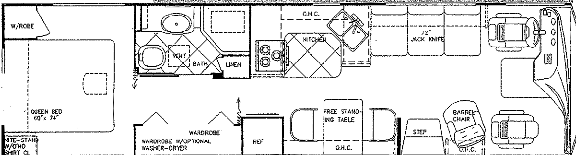
Model 8349 MXG (Approx 33'-8" 101" Wide)
