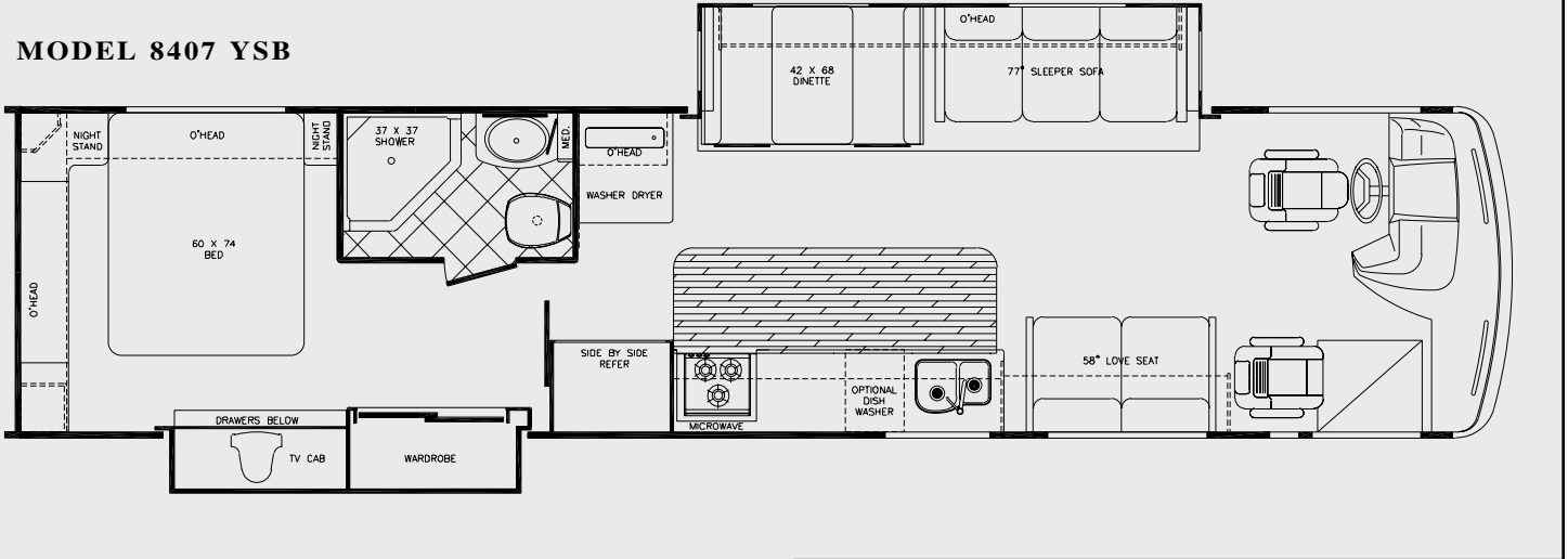
MODEL 8407, YSB
