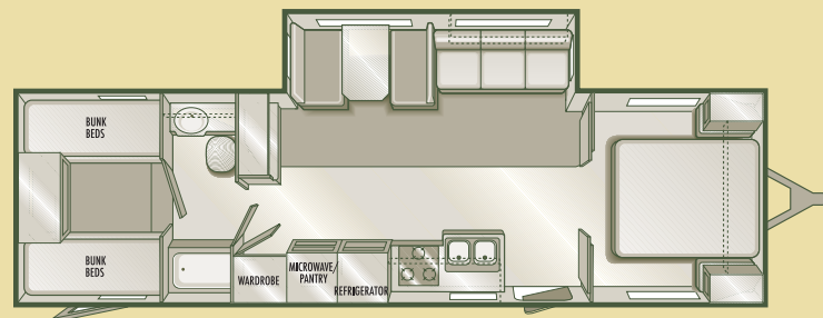
3310 TRAVEL TRAILER Available with Options: F, N, S and T
