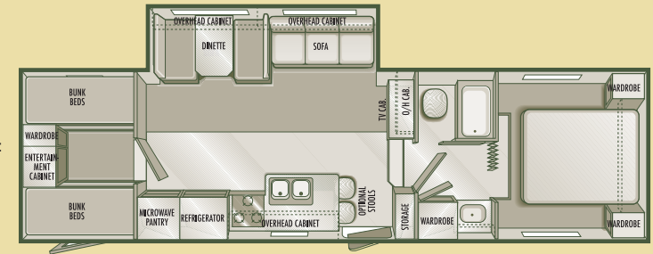
3150 FIFTH WHEEL Available with Options: F, N and V
