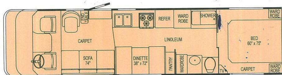
LAND YACHT 33' queen or twin bed options
